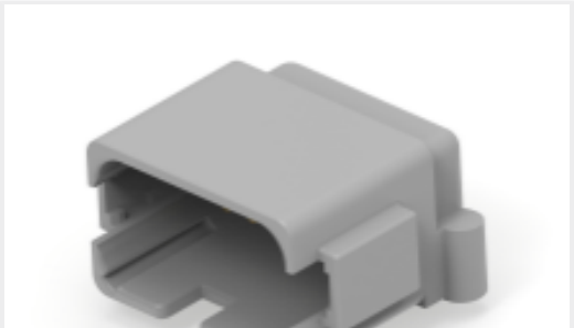
TE Part #DTF13-12PA-G003 HDR, 12P, GRY, RA, AU/NI/CU, A
