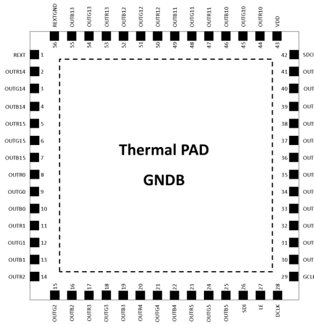
MBI5353GFN
