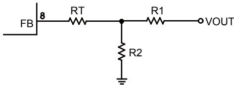
Figure 6: T-Type Network
