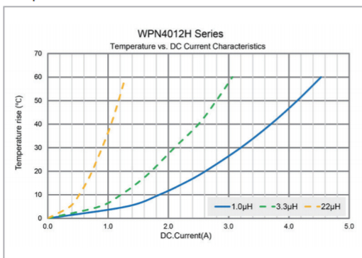
WPN4012H Series Temperature vs. DC Current Characteristics
