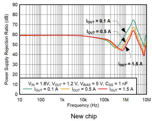
Figure 5-16. V_{BIAS} PSRR vs Frequency New chip
