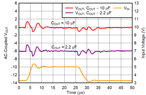
Figure 7-12. V_{BIAS} Line Transient
