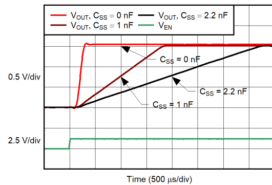
Figure 7-6. Turn-On Response
