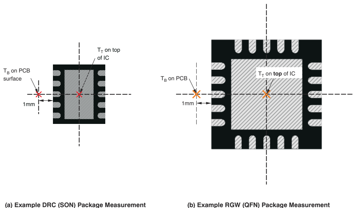
Figure 7-14. Measuring Points for T_T and T_B
