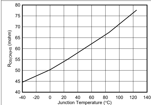
Figure 6-5. High-Side R_{DS(ON)}
