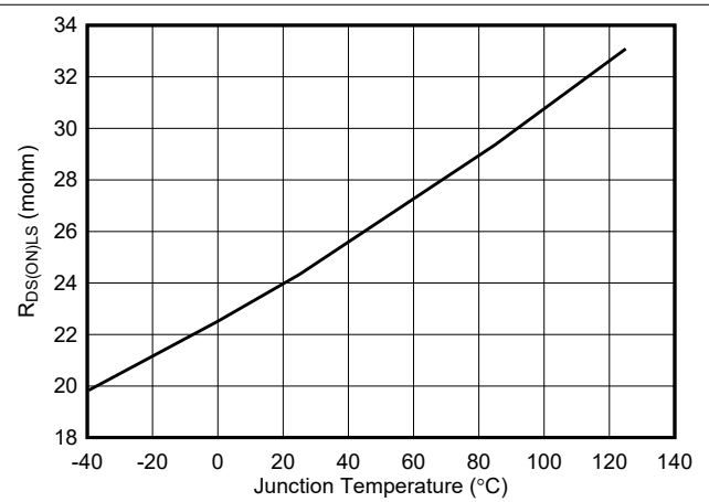
Figure 6-4. Low-Side R_{DS(ON)}
