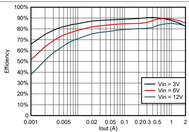
Figure 6-8. Efficiency at 1.05 V OUT with a 1.2- \mu\text{H} Inductor
