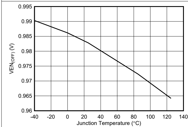
Figure 6-3. Enable Off Threshold Voltage
