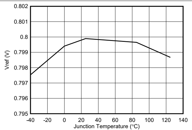
Figure 6-6. V_{REF} Voltage
