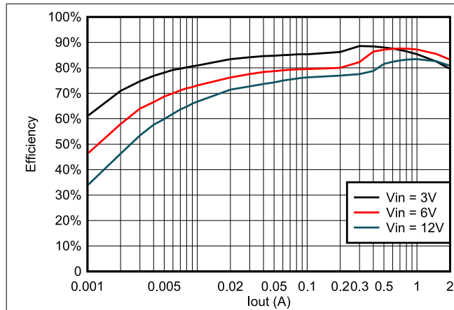
Figure 6-7. Efficiency at 0.8 V OUT with a 1- \mu\text{H} Inductor
