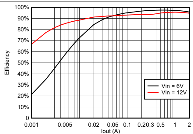
Figure 6-10. Efficiency at 5 V OUT with a 3.3- \mu\text{H} Inductor
