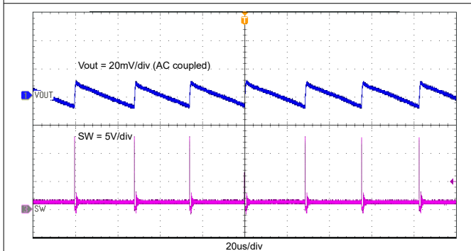
Figure 8-6. Output Voltage Ripple with 0.01-A Loading
