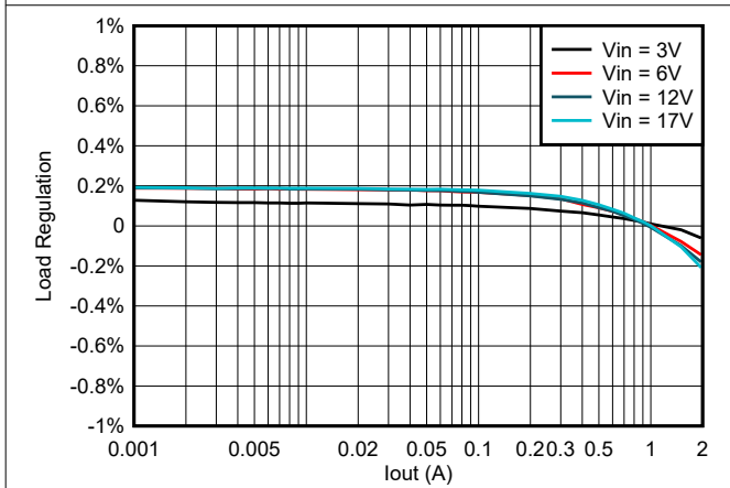
Figure 8-4. Load Regulation vs Loading
