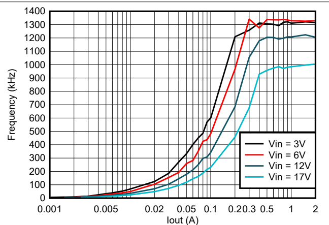
Figure 8-3. Frequency vs Loading
