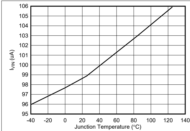
Figure 6-1. Quiescent Current
