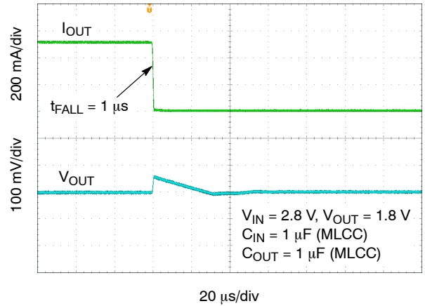
Figure 33. Load Transient Response – 450 mA to 1 mA – V_{OUT} = 1.8 V
