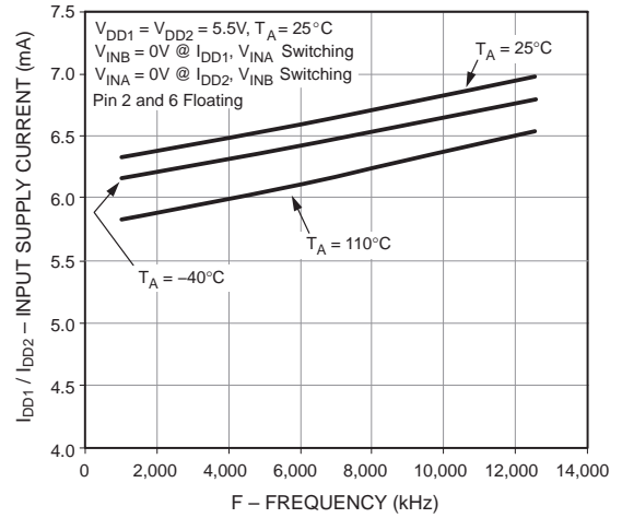
Figure 13. Typical I_{DD1}/I_{DD2} Supply Current vs. Frequency
