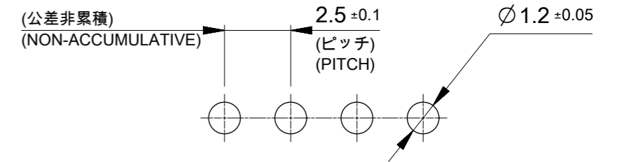
基板取付穴推奨寸法 RECOMMENDED P.C. BOARD HOLE DIM.
