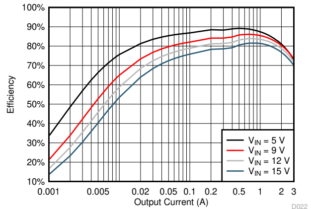
Figure 7-5. TPS563201 Efficiency
