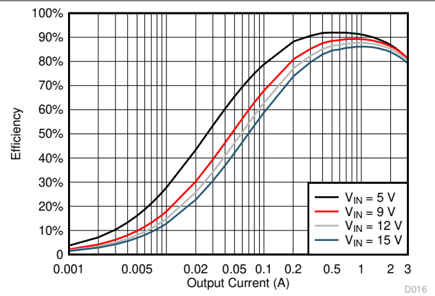
Figure 5-16. TPS563208 V_{OUT} = 1.8\text{ V} Efficiency, L = 2.2\ \mu\text{H}
