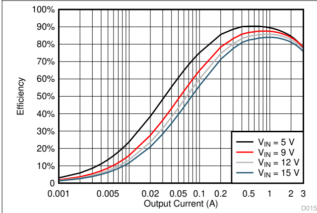
Figure 5-15. TPS563208 V_{OUT} = 1.5\text{ V} Efficiency, L = 2.2\ \mu\text{H}
