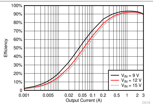
Figure 5-18. TPS563208 V_{OUT} = 5\text{ V} Efficiency, L = 3.3\ \mu\text{H}
