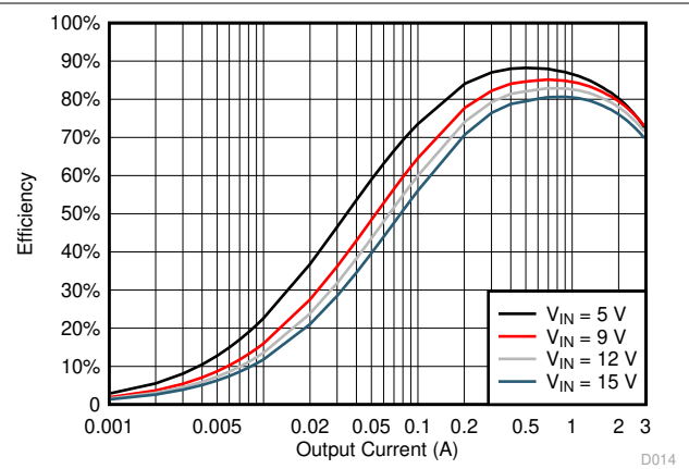
Figure 5-14. TPS563208 V_{OUT} = 1.05\text{ V} Efficiency, L = 2.2\ \mu\text{H}
