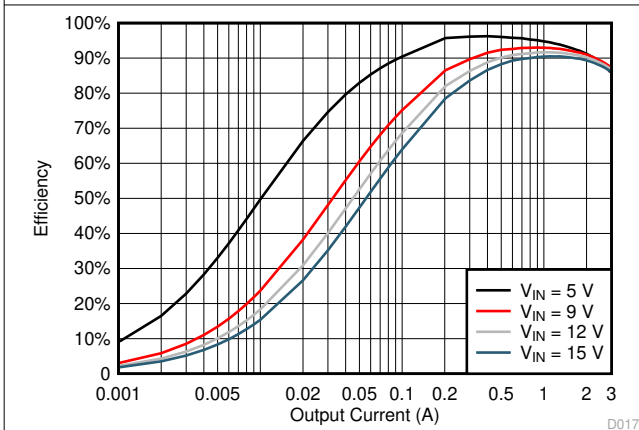
Figure 5-17. TPS563208 V_{OUT} = 3.3\text{ V} Efficiency, L = 2.2\ \mu\text{H}
