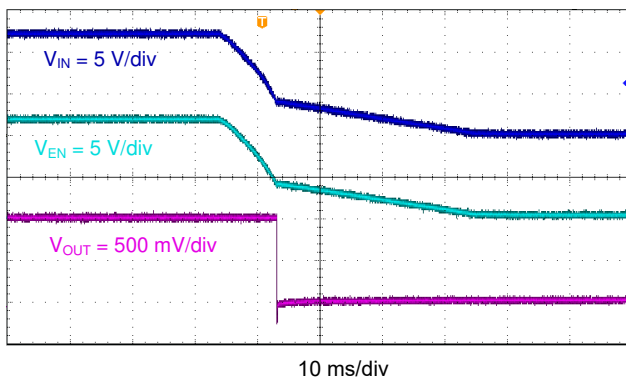
Figure 7-16. TPS563201 Shutdown Relative to V_I
