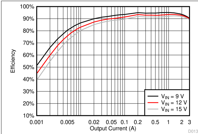
Figure 5-13. TPS563201 V_{OUT} = 5\text{ V} Efficiency, L = 3.3\ \mu\text{H}
