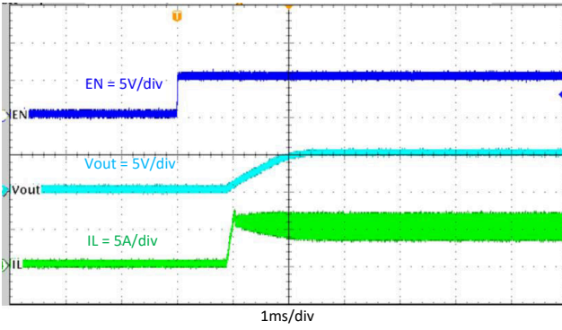
Figure 8-8. Start-Up Through EN, I_{OUT} = 5\text{ A}
