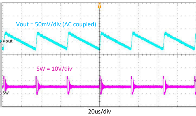
Figure 8-12. Output Voltage Ripple, I_{OUT} = 0.1\text{ A}
