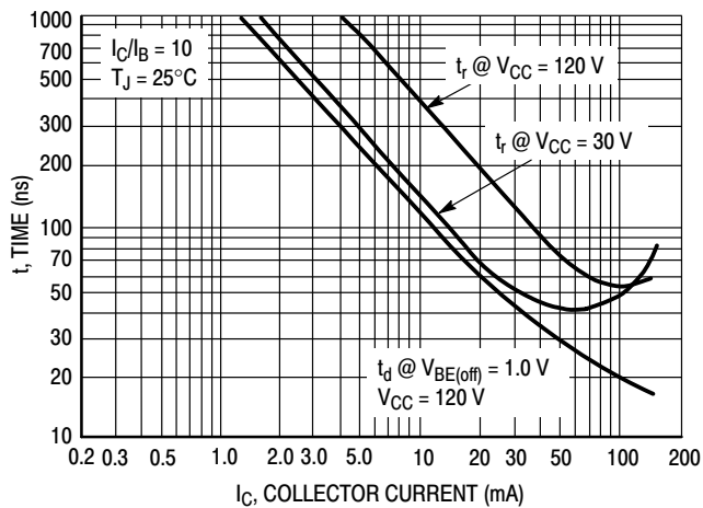
Figure 10. Turn-On Time
