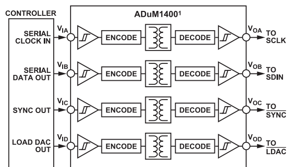
Figure 62. Isolated Interface
