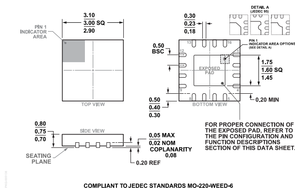
Figure 63. 16-Lead Lead Frame Chip Scale Package [LFCSP] 3 mm × 3 mm Body and 0.75 mm Package Height (CP-16-22) Dimensions shown in millimeters
