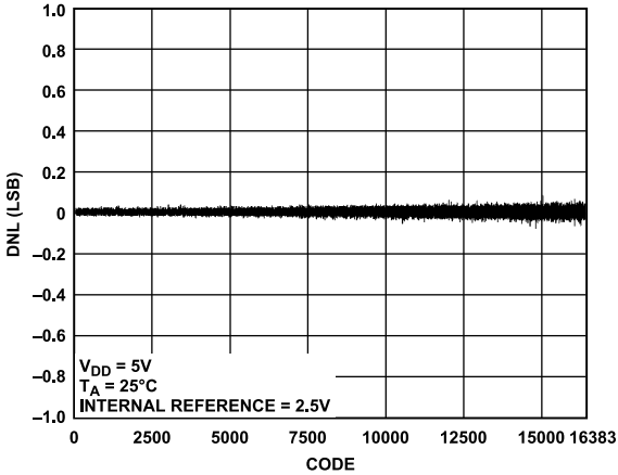
Figure 19. AD5685R DNL
