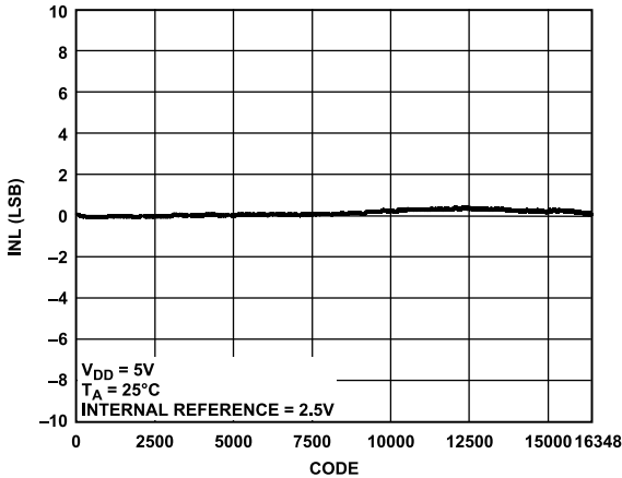
Figure 16. AD5685R INL
