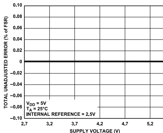
Figure 29. TUE vs. Supply, Gain = 1
