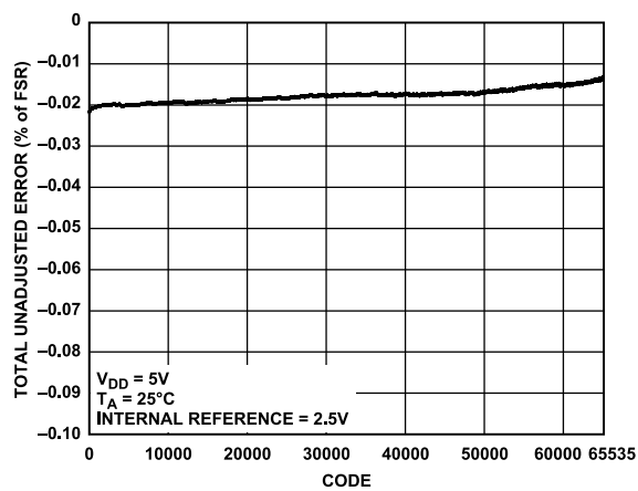
Figure 30. TUE vs. Code
