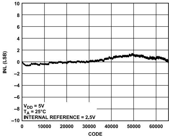
Figure 15. AD5686R INL
