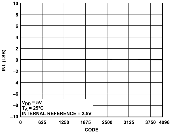
Figure 17. AD5684R INL
