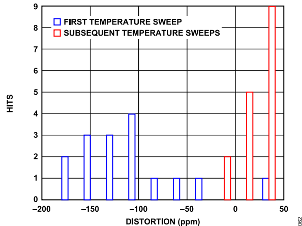
Figure 57. Thermal Hysteresis
