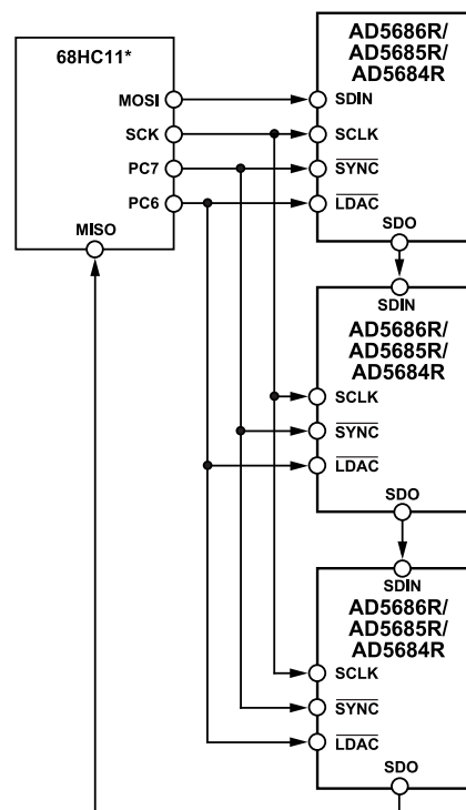
Figure 53. Daisy-Chaining the AD5686R/AD5685R/AD5684R
