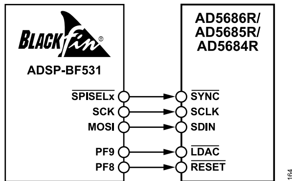
Figure 59. ADSP-BF531 Interface
