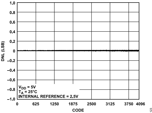
Figure 20. AD5684R DNL
