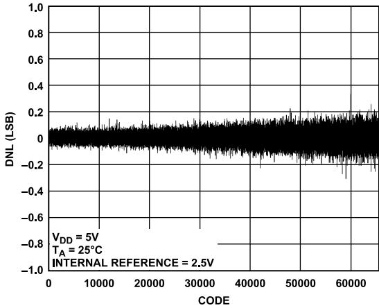
Figure 18. AD5686R DNL
