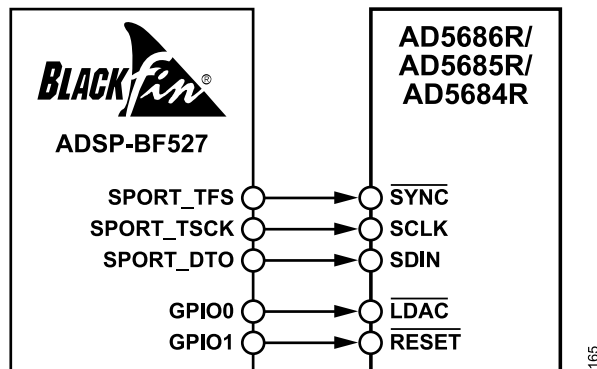
Figure 60. SPORT Interface
