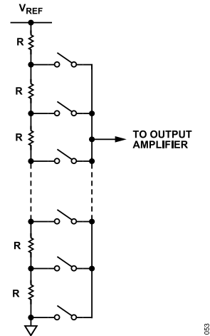
Figure 49. Resistor String Structure
