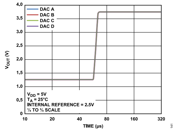
Figure 37. Settling Time, 5.25 V
