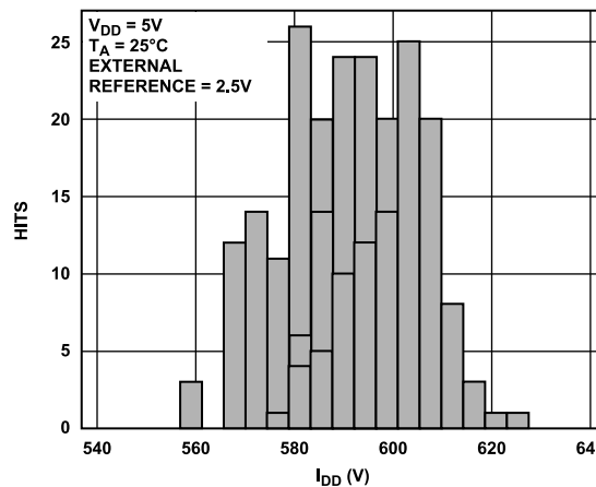
Figure 31. I_{DD} Histogram with External Reference, 5 V
