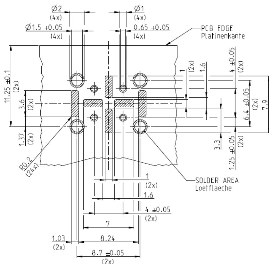
Figure / Bild 4: PCB Layout for MATE-AX header 2304168
