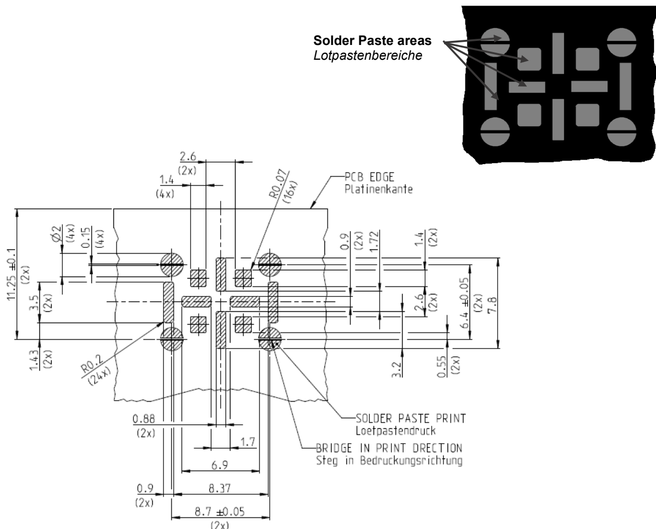
Figure / Bild 5: Solder paste layout for MATE-AX header 2304168
