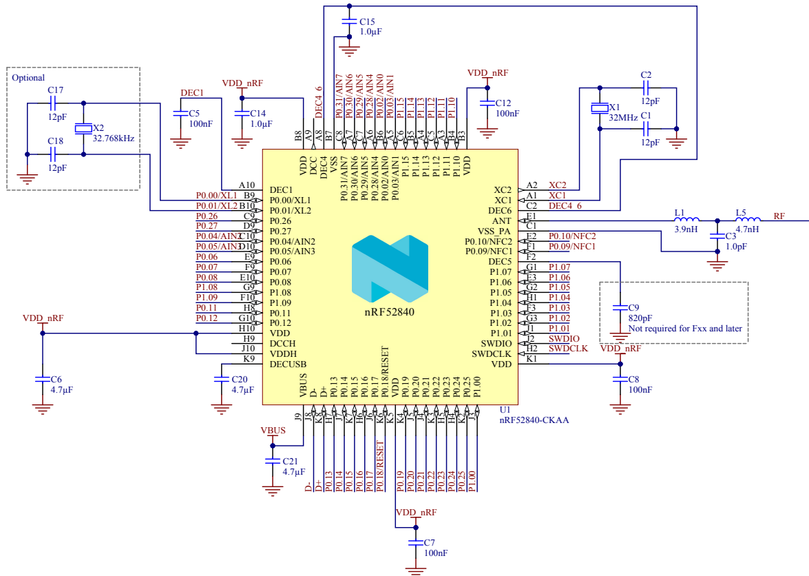
Figure 223: Circuit configuration no. 3 schematic for CKA WLCSP
