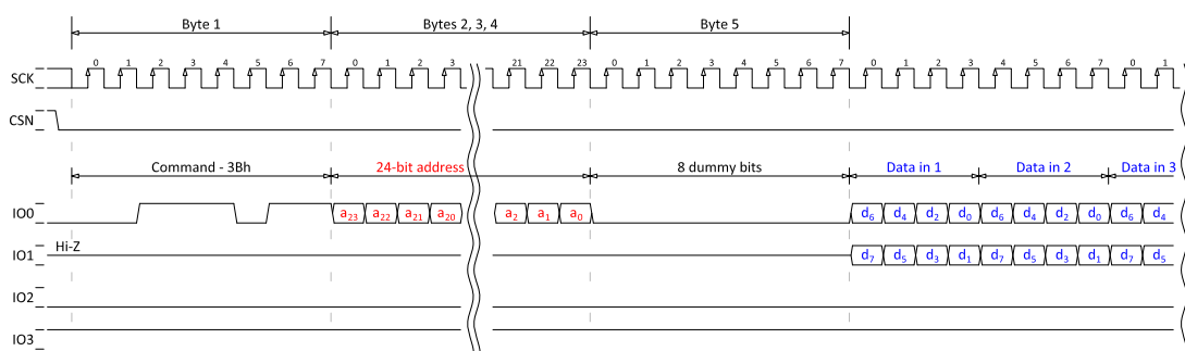
Figure 90: 24-bit READ2O (dual-read output), SPI MODE = MODE0
