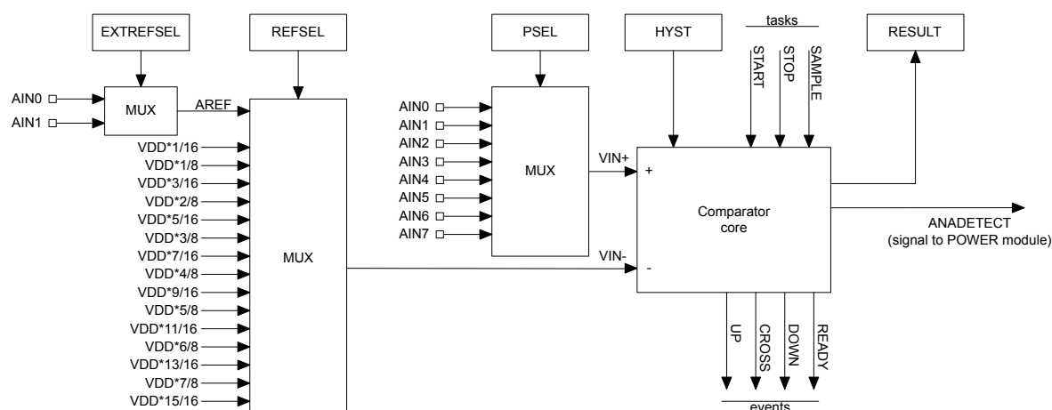
Figure 59: Low-power comparator
