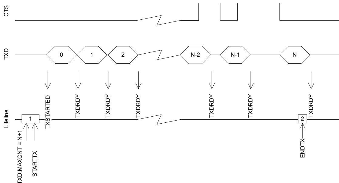
Figure 192: UARTe transmission
