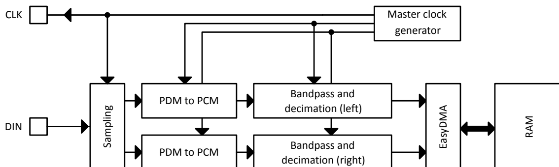
Figure 70: PDM module
