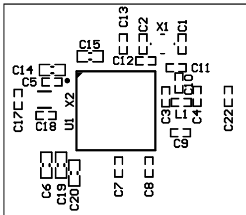
Figure 227: Top silk layer
