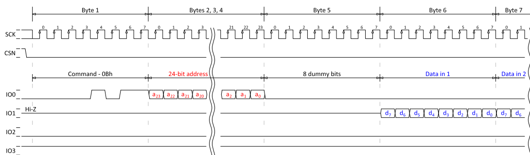
Figure 89: 24-bit FASTREAD, SPI MODE = MODE0
