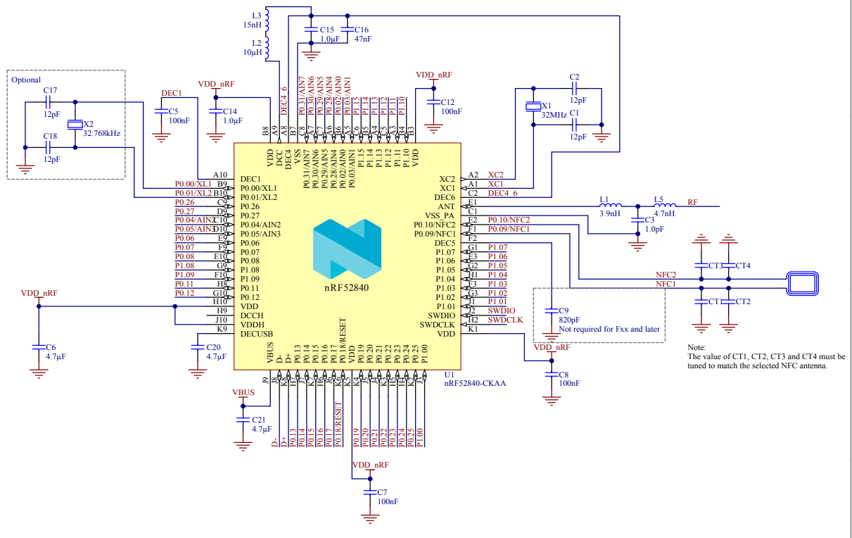
Figure 225: Circuit configuration no. 5 schematic for CKAA WLCSP
