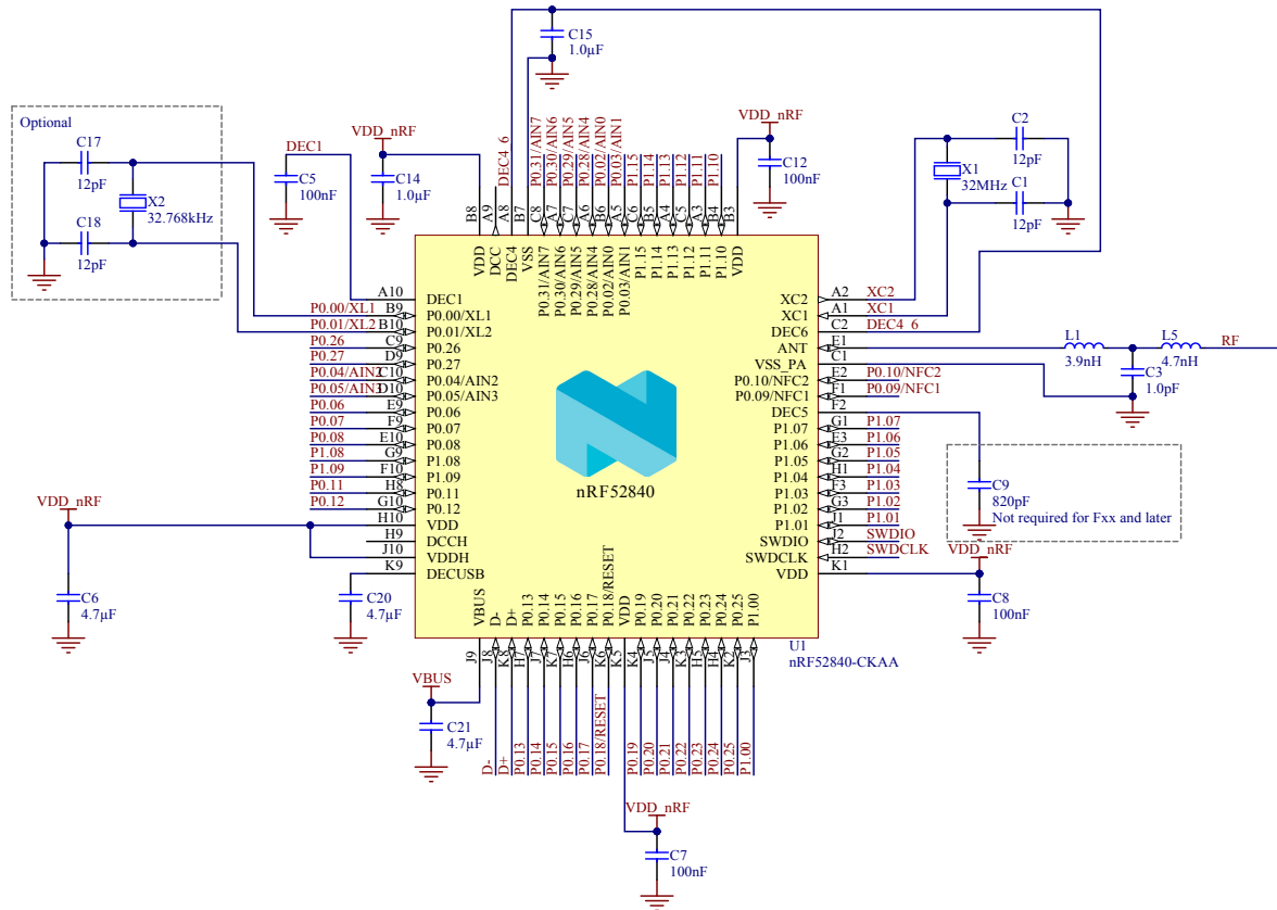
Figure 223: Circuit configuration no. 3 schematic for CKA WLCSP
