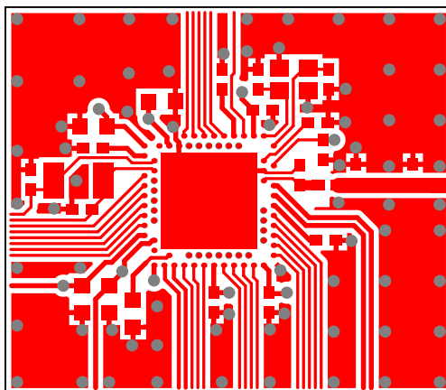
Figure 228: Top layer
