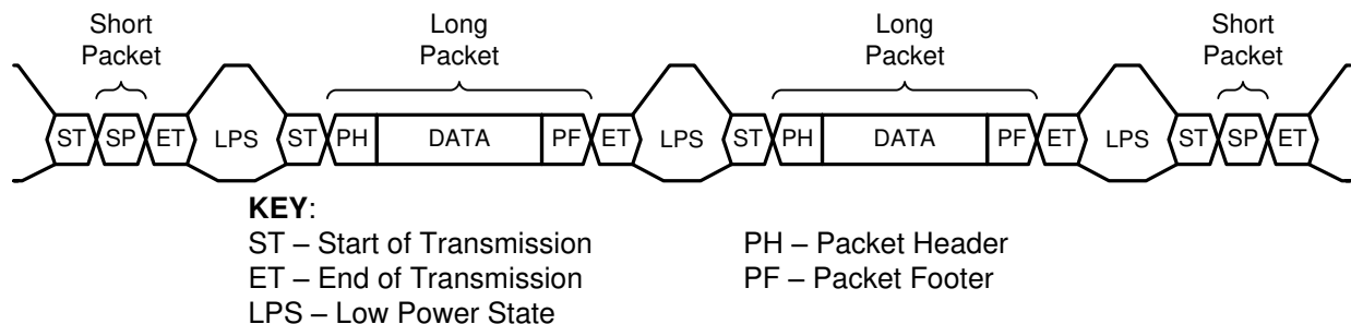
Figure 7-8. CSI-2 Protocol Layer With Short and Long Packets
