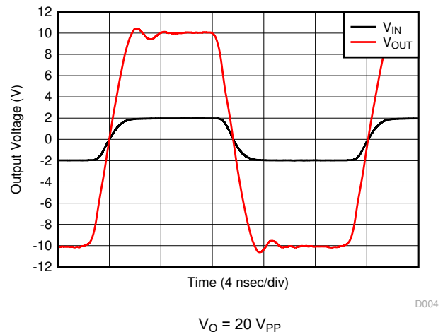
Figure 8-24. G = 5 V/V Pulse Response
