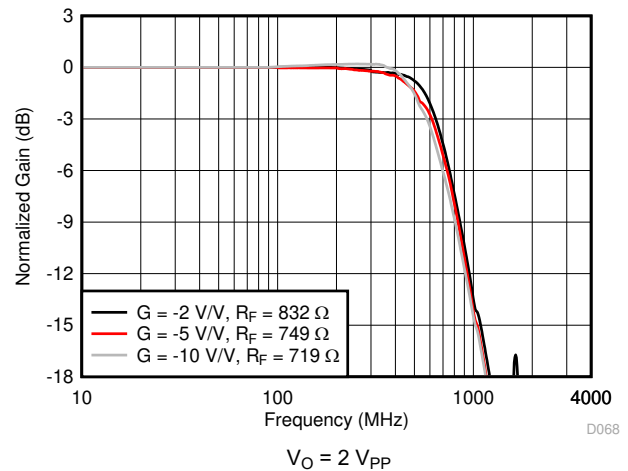
Figure 8-43. Inverting Small-Signal Frequency Response
