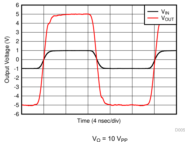
Figure 8-23. G = 5 V/V Pulse Response
