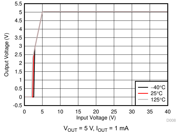
Figure 6-8. Output Voltage vs Input Voltage
