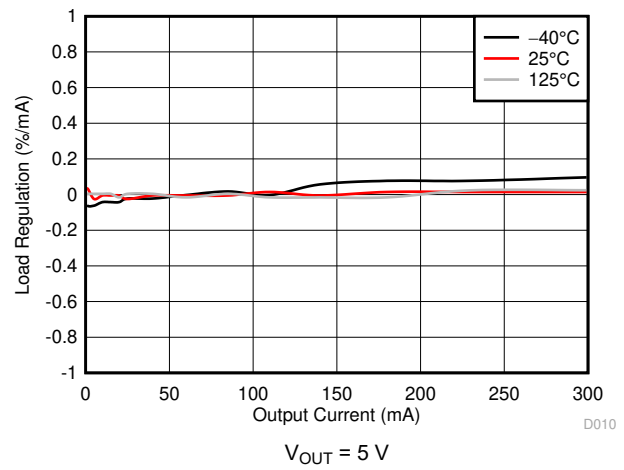
Figure 6-10. Load Regulation
