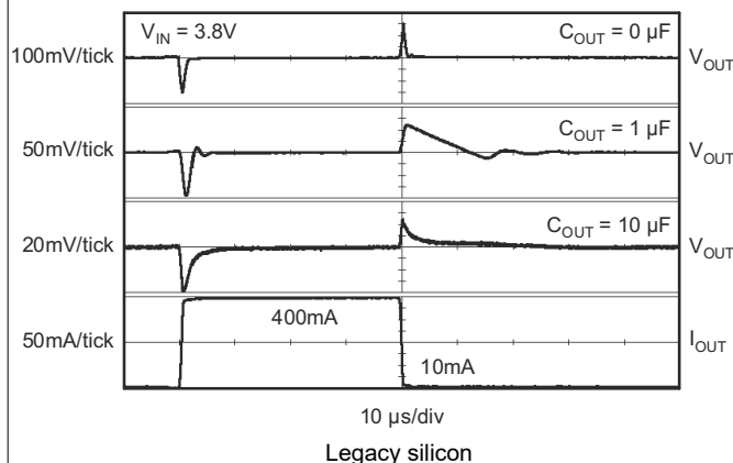
Figure 5-35. TPS73633 Load Transient Response
