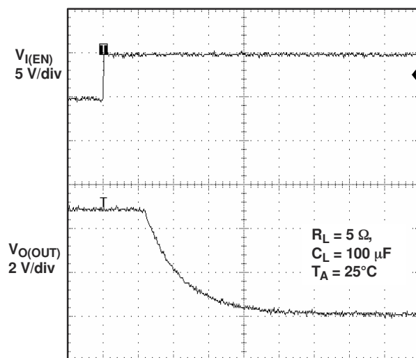
Figure 6-33. Turnoff Delay and Fall Time With 100-μF Load
