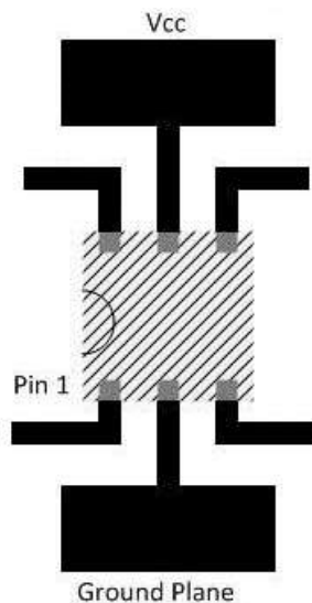
Figure 17-1. Recommended Layout Example
