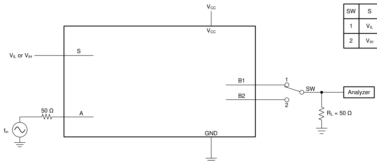
Figure 13-7. Feed Through
