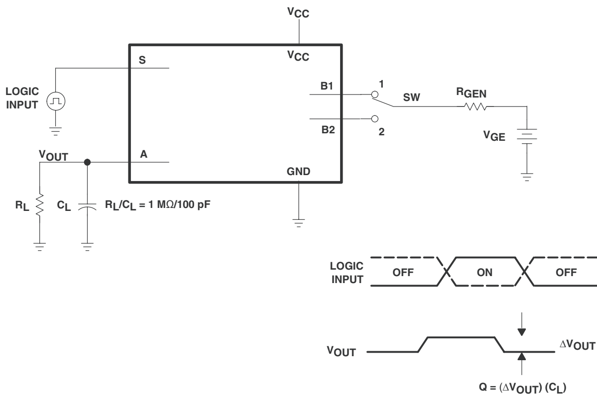
Figure 13-8. Charge-Injection Test
