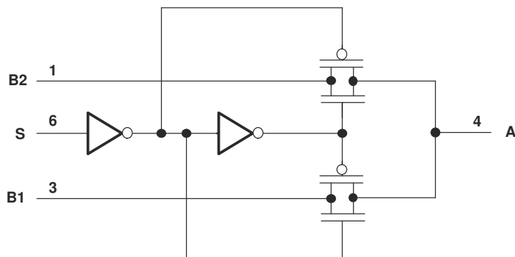
Figure 14-1. Logic Diagram (Positive Logic)
