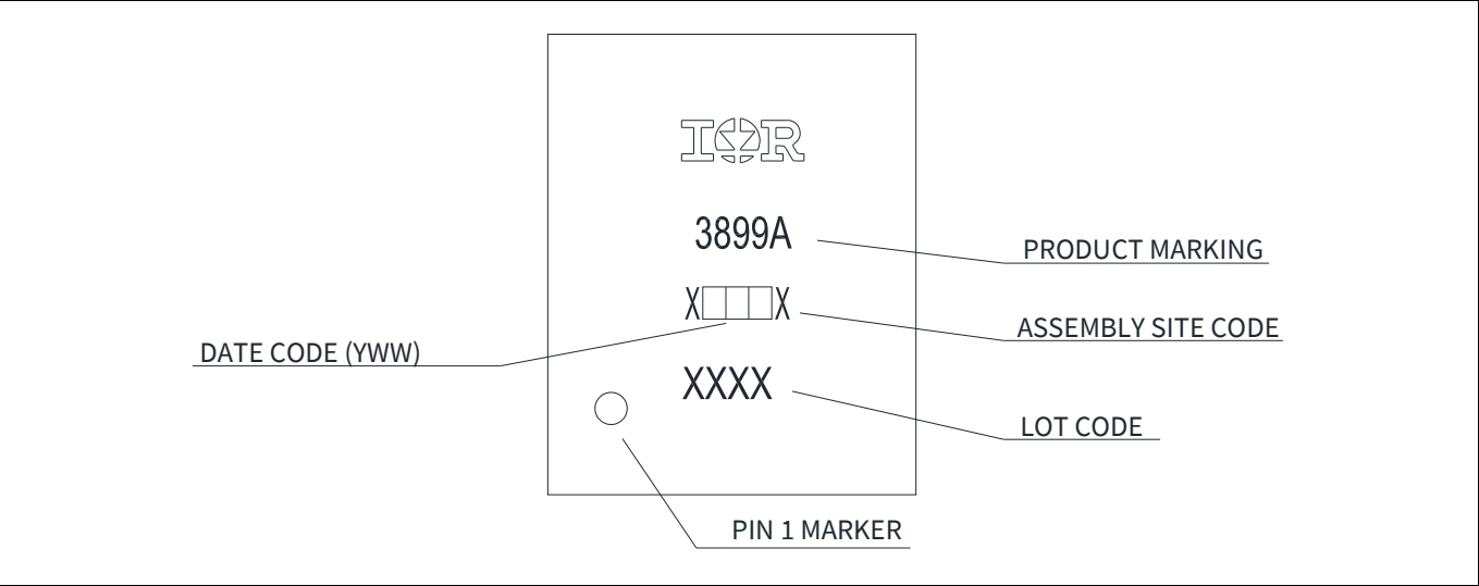
Figure 22 Package Marking
