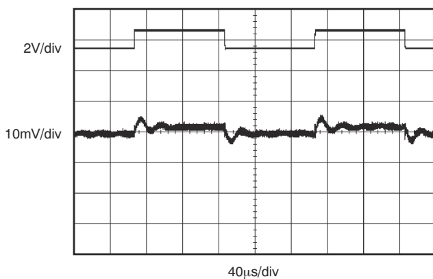
Figure 5-31. Step Response
