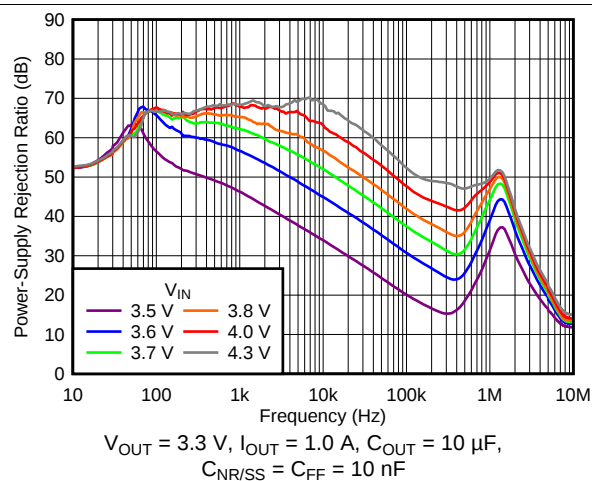
Figure 3. PSRR vs Frequency and Input Voltage
