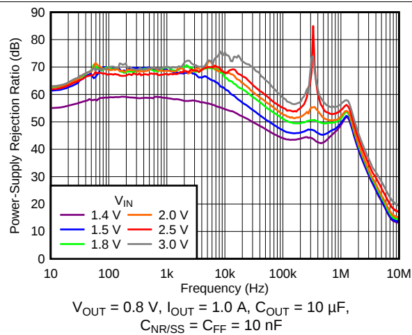
Figure 1. PSRR vs Frequency and Input Voltage
