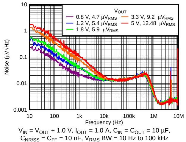
Figure 8. Spectral Noise Density vs Frequency and Output Voltage
