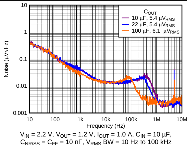
Figure 11. Spectral Noise Density vs Frequency and C_{OUT}
