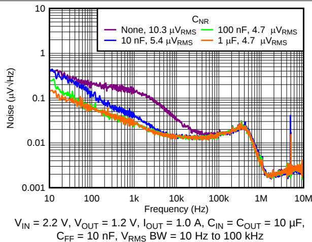
Figure 9. Spectral Noise Density vs Frequency and C_{NR/SS}
