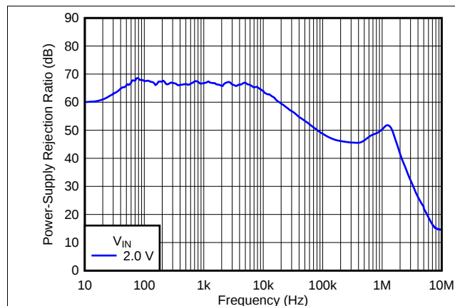
Figure 40. PSRR vs Frequency
