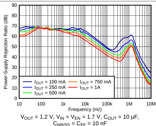
Figure 5. PSRR vs Frequency and Output Current
