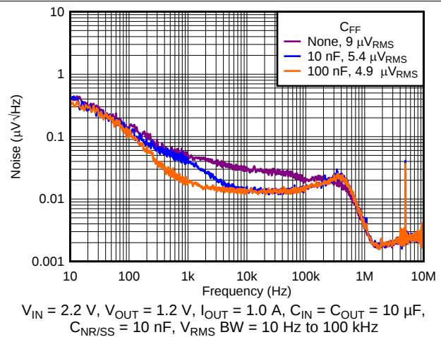
Figure 10. Spectral Noise Density vs Frequency and C_{FF}
