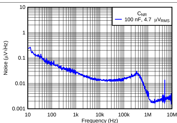
Figure 41. Output Noise vs Frequency
