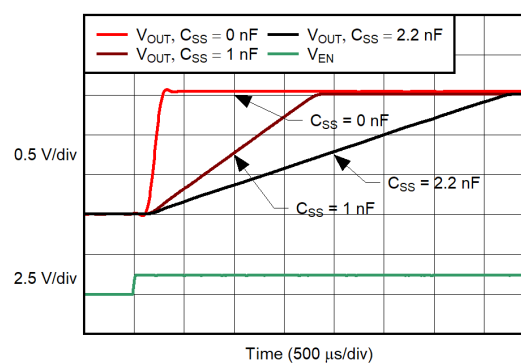
Figure 7-6. Turn-On Response
