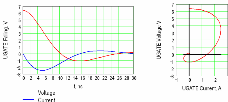
Figure 7-6. UGATE Turning Off Voltage and Sink Current vs Time (Related Switching Diagram (right))
