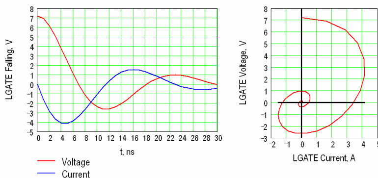
Figure 7-5. LGATE Turning Off Voltage and Sink Current vs Time (Related Switching Diagram (right))
