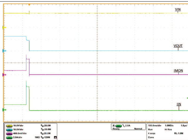
Figure 33. TPS2595x0 Overcurrent Response
