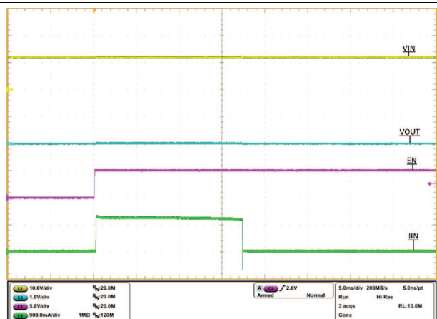
Figure 34. Output Hot Short to GND Response
