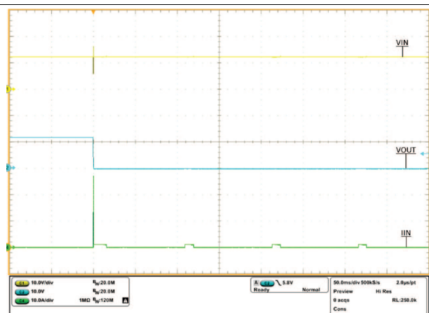
Figure 32. TPS2595x1, TPS2595x3, TPS2595x5 OverCurrent Response
