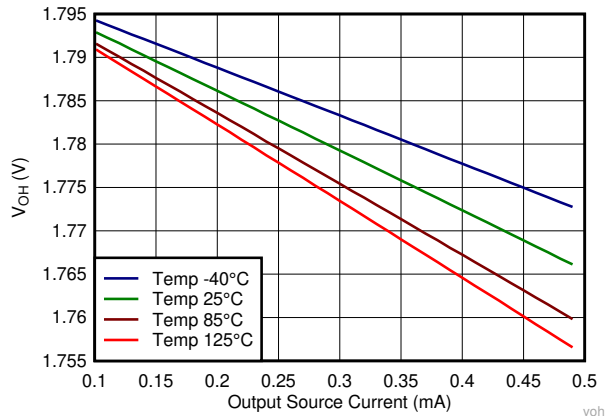
V_{CC} = 1.8\text{V} TLV703x
