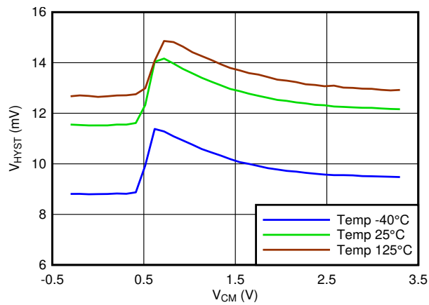
V_{CC} = 3.3\text{V} TLV70x2
