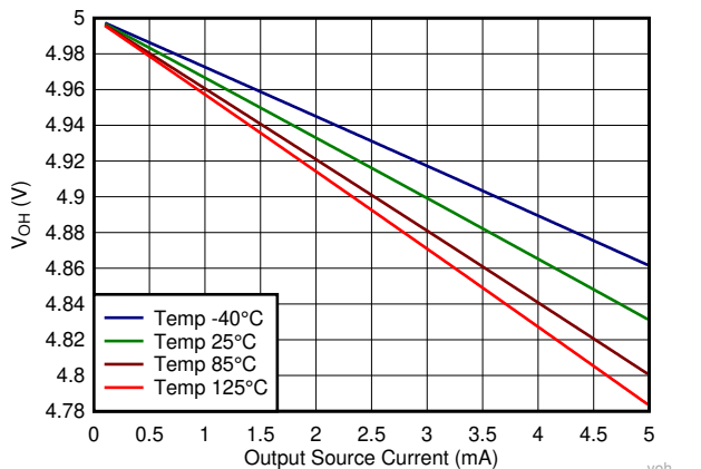
V_{CC} = 5\text{V} TLV703x
