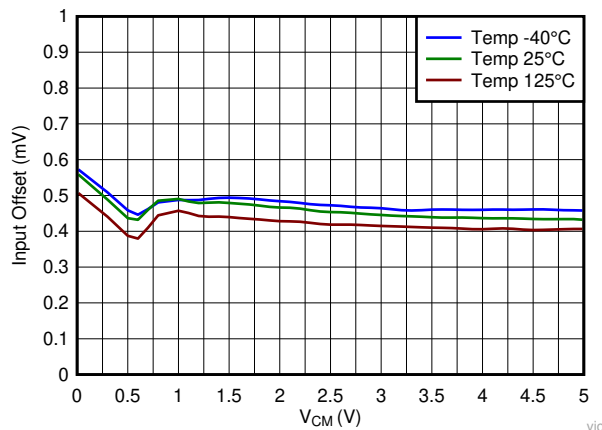
Figure 5-6. Input Offset Voltage vs V_{CM}
