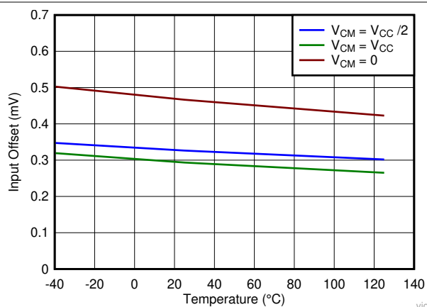
Figure 5-4. Input Offset vs Temperature
