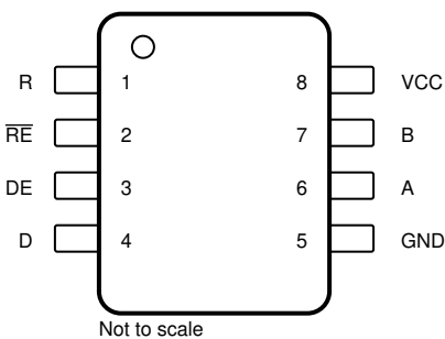
Figure 5-1. D (SOIC) and DGK (VSSOP), 8-Pin Packages, Top View
