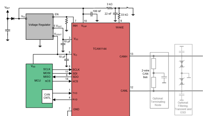
Simplified Schematics
