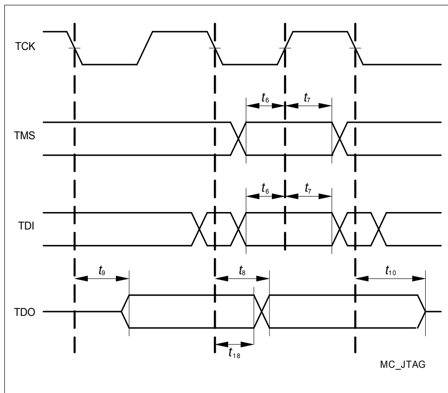
Figure 14 JTAG Timing
