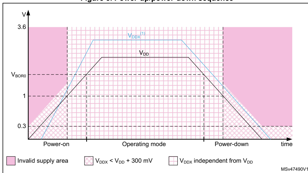
Figure 3. Power-up/power-down sequence
