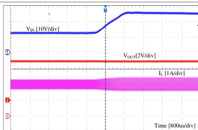
Figure 9-7. Line Transient
