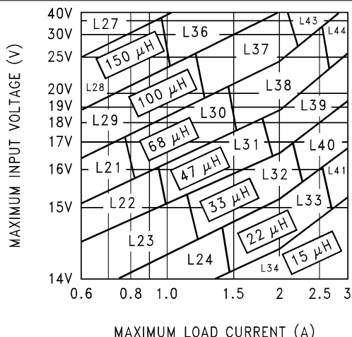
Figure 9-7. LM2596-12
