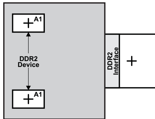
Figure 7-42. DDR2 Keepout Region
