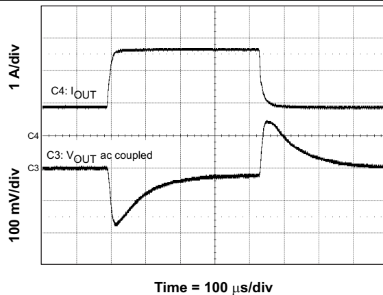
Figure 35. Load Transient
