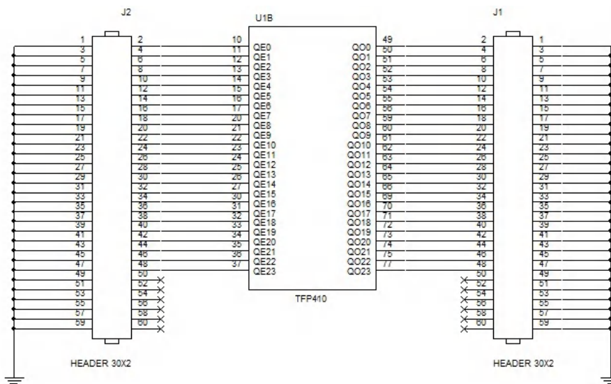
Figure 7-2. Data Signals
