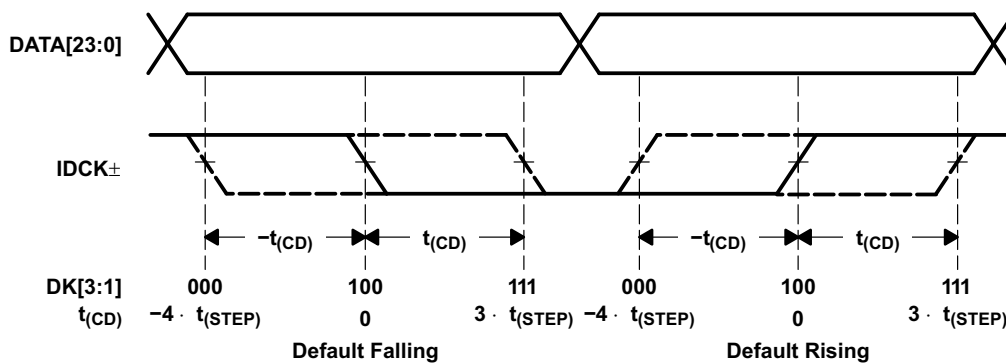
Figure 6-3. A Graphical Representation of the De-Skew Function
