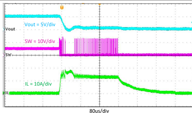
Figure 8-17. Normal Operation to Output Hard Short
