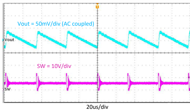
Figure 8-12. Output Voltage Ripple, I_{OUT} = 0.1\text{ A}
