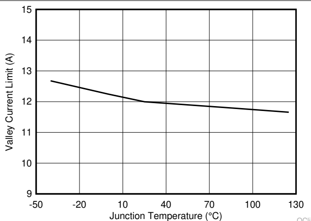
Figure 6-11. Valley Current Limit vs Junction Temperature
