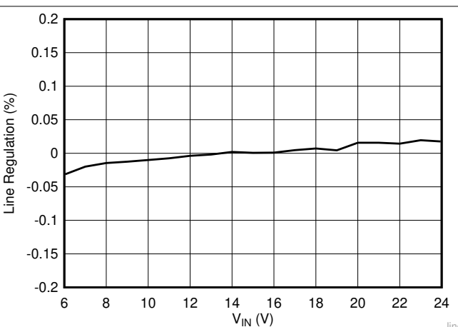
Figure 8-6. Line Regulation, I_{OUT} = 0.1\text{ A}
