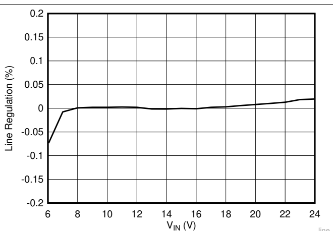
Figure 8-7. Line Regulation, I_{OUT} = 5\text{ A}
