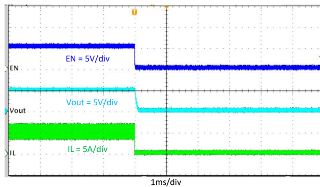
Figure 8-9. Shut-down Through EN, I_{OUT} = 5\text{ A}
