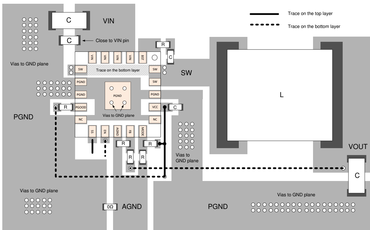
Figure 10-1. Top-Side Layout
