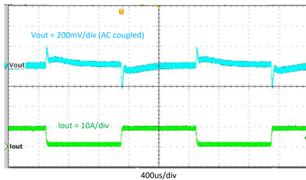
Figure 8-15. Transient Response, 1 A to 9 A, Slew Rate = 2.5 A/μs
