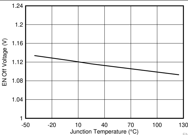
Figure 6-5. Enable Off Voltage vs Junction Temperature
