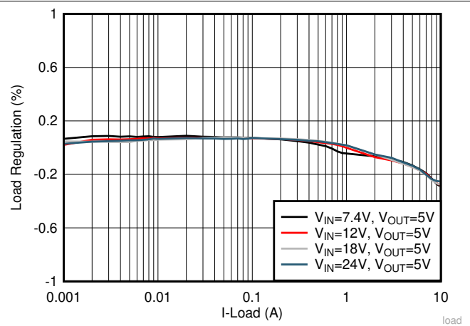
Figure 8-3. Load Regulation
