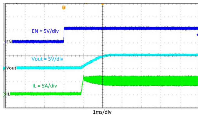
Figure 8-8. Start-Up Through EN, I_{OUT} = 5\text{ A}
