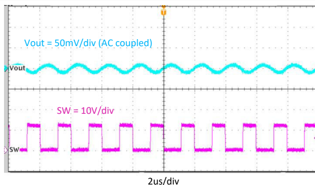
Figure 8-13. Output Voltage Ripple, I_{OUT} = 5\text{ A}
