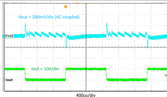
Figure 8-16. Transient Response, 0 A to 10 A, Slew Rate = 2.5 A/μs
