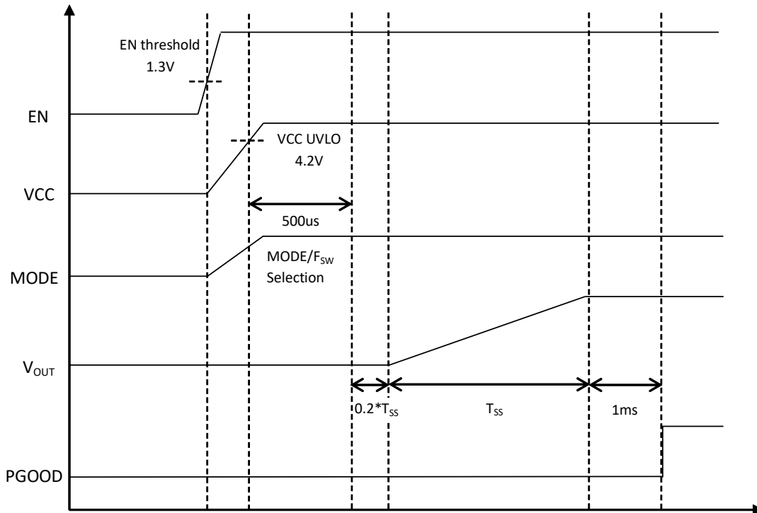
Figure 7-1. Power-Up Sequence
