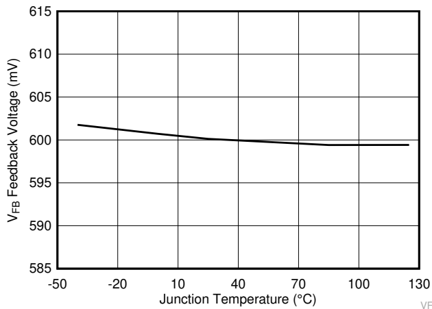
Figure 6-3. Feedback Voltage vs Junction Temperature
