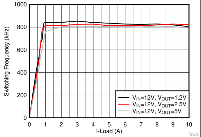
Figure 6-20. Switching Frequency vs Load Current, F_{SW} = 800 kHz, Eco-mode
