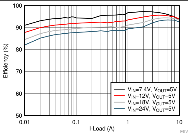
Figure 8-2. Efficiency Curve
