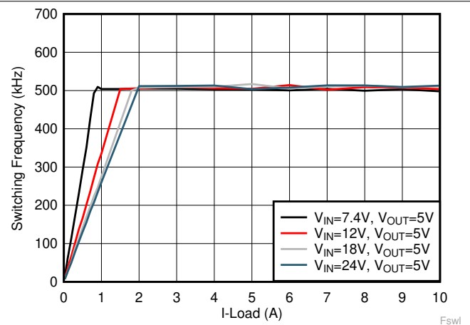
Figure 8-5. Switching Frequency vs Output Load
