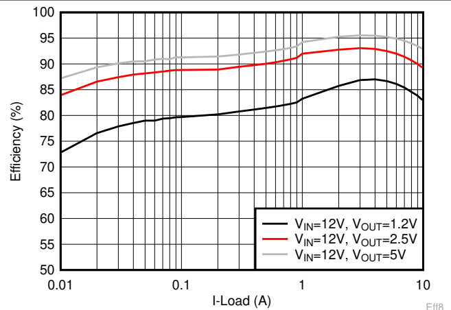
Figure 6-16. Efficiency vs Load Current, F_{SW} = 800 kHz, Eco-mode
