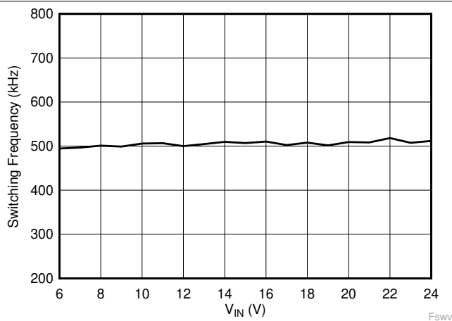
Figure 8-4. Switching Frequency vs Input Voltage, I_{OUT} = 5\text{ A}
