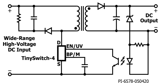
Figure 1. Typical Standby Application.
