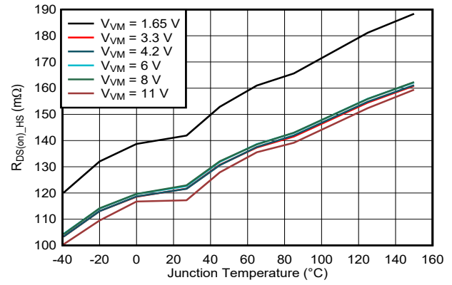
Figure 7-22. High-Side R_{DS(on)} vs. Junction Temperature ( T_J )
