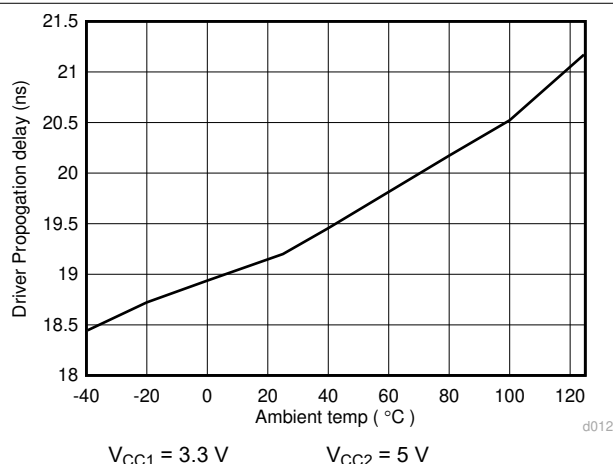
Figure 7-21. ISO145x Driver Propagation Delay (ns) Vs Temperature (C)
