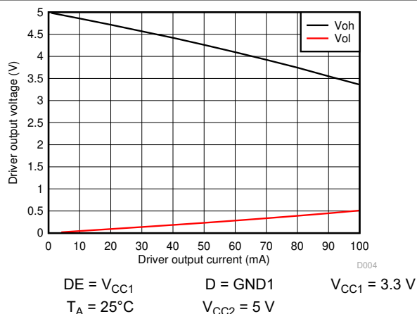
Figure 7-12. Driver Output Voltage Vs Driver Output Current
