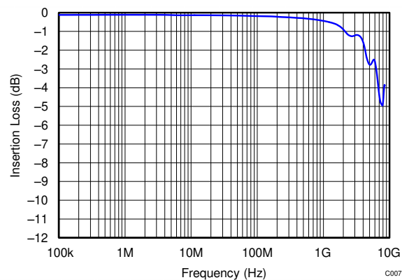
Figure 6-8. TPD1E05U06 Insertion Loss
