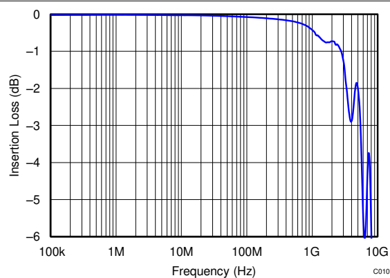
Figure 6-8. TPD1E05U06 Insertion Loss
