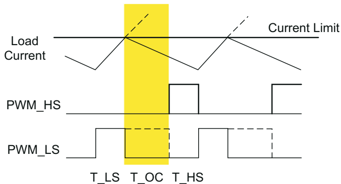
Figure 6-2. Cycle-by-Cycle Operation With Low-Side OC
