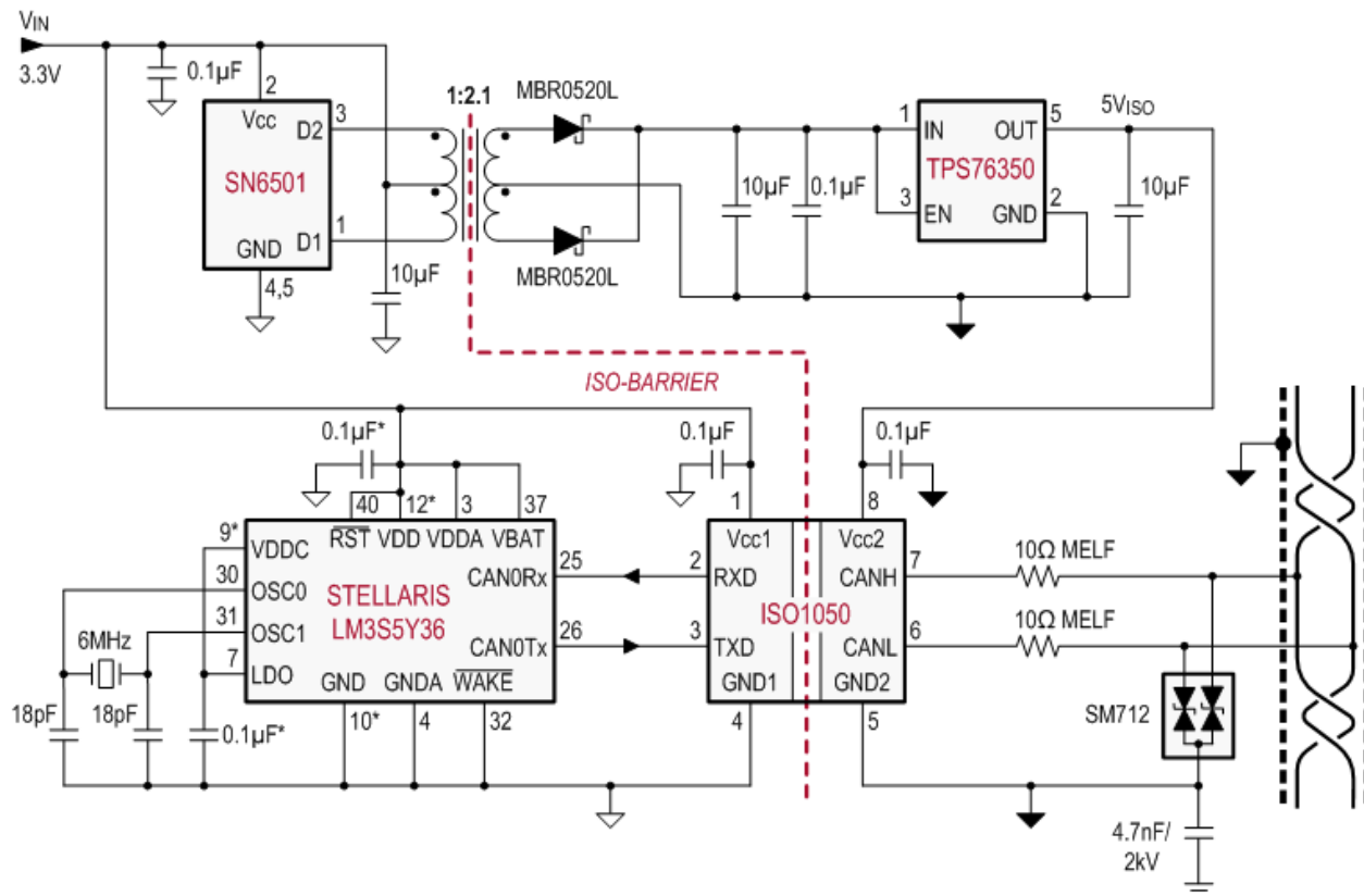
Figure 8-13. Isolated Can Interface
